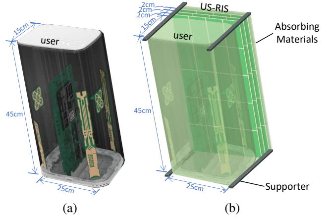
Fig. 2. Illustration of user architecture. (a) A real-world CPE. (b) The proposed user architecture equipped with a multi-layer US-RIS.
